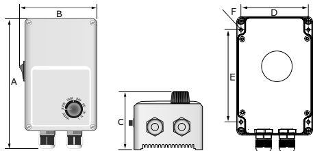
Fig. 5 Mounting dimensions
