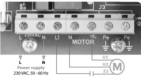
Fig. 4 Operational diagram
